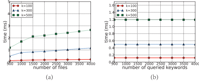
Figure 9: (a) The time to select the top- k files' identifiers on different scale of file sets. (b) The time to select the top- k files' identifiers for different number of queried keywords, the number of files in the file set is n = 500 .
